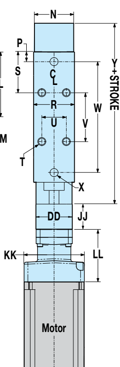
RIP Motor Mount
