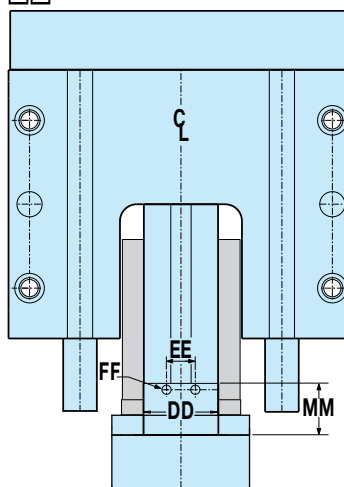
RIP Motor Mount
