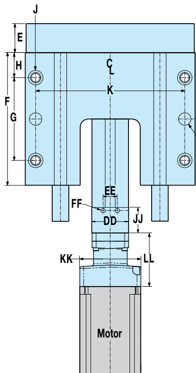
LMI Motor Mount
