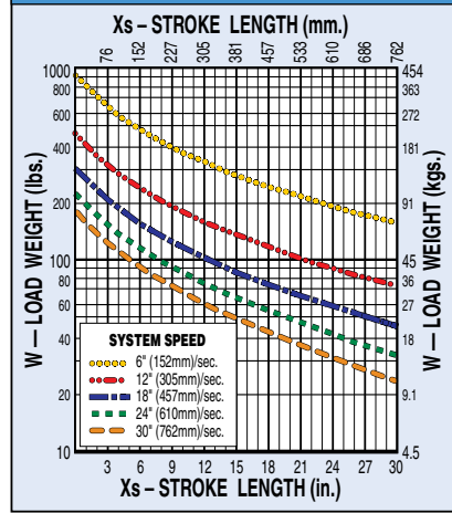
MAXIMUM LOAD WEIGHT vs STROKE LENGTH COMPOSITE BEARING, OVERSIZE GUIDE RODS
